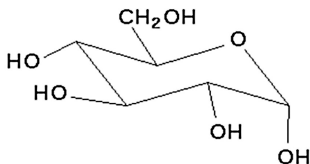
Figure 3. Chemical structure of a glucose molecule.
